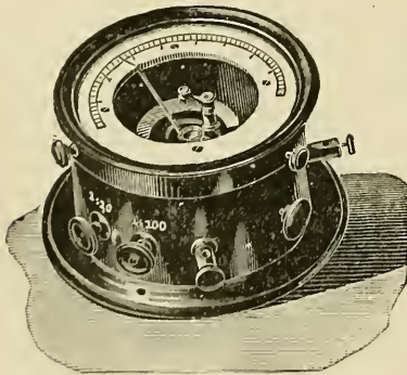
FIG. 103. — Edelmann galvanometer.
